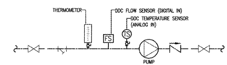
F1 TYPICAL DDC MONITORING AT HW RECIRCULATION & CW CIRCULATION PUMPS SCALE: NONE
