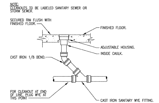
C9 FLOOR CLEANOUT DETAIL SCALE: NONE
