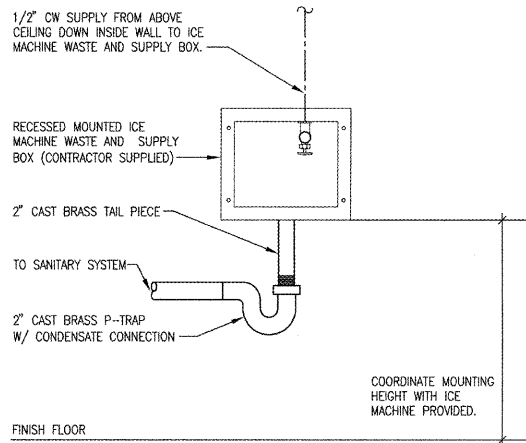
B4 ICE MAKER SUPPLY BOX DETAIL SCALE: NONE
