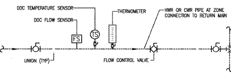
E6 TYPICAL DDC MONITORING AT HW RECIRCULATION & CW CIRCULATION ZONES SCALE: NONE
