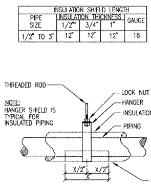
B6 INSULATION SHIELD DETAIL SCALE: NONE
