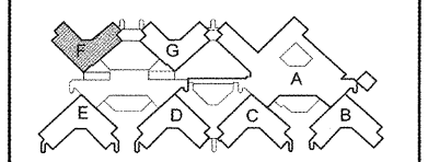
"F" WING SECOND FLOOR PARTIAL ARCHITECTURAL DIMENSION FLOOR PLAN SCALE: 1/4" = 1'-0"
