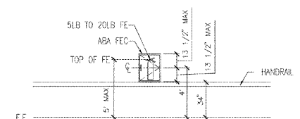
F4 TYPICAL MOUNTING HEIGHTS SCALE: 1/4" = 1'-0"
