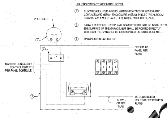
5 LIGHTING CONTACTOR DETAIL N.T.S.
