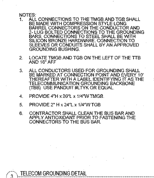
3 TELECOM GROUNDING DETAIL N.T.S.
