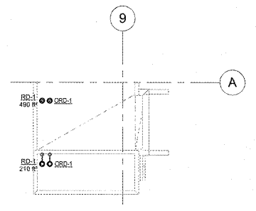
3 ELEV./STAIR 1 PARTIAL ROOF PLAN PP103 3/32" = 1'-0"
