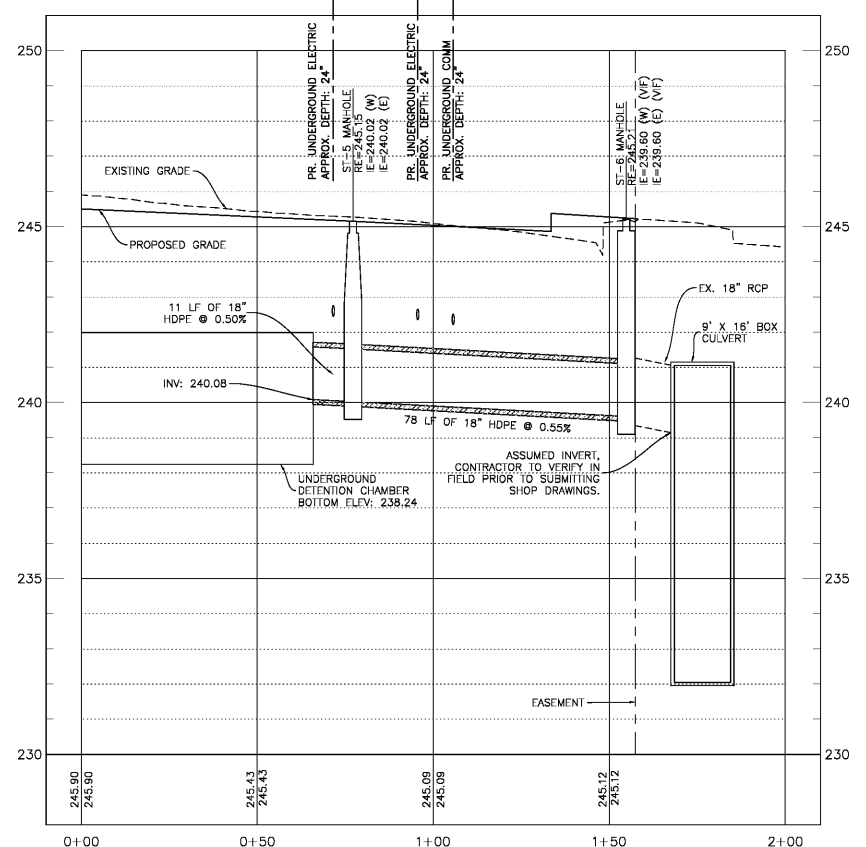
STORM CENTERLINE PROFILE HOR. SCALE 1" = 20' VERT. SCALE 1" = 2'
