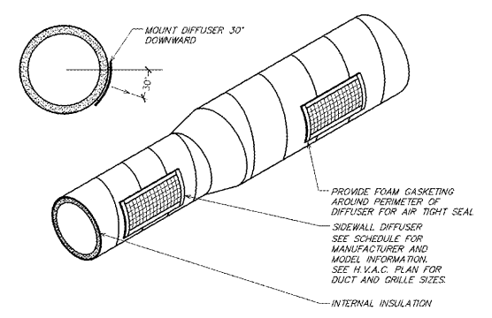
3 DUCT MOUNTED DIFFUSER DETAIL SCALE: NONE
