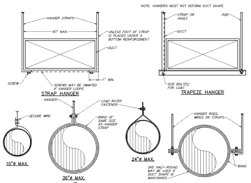
11 DUCT HANGER DETAIL SCALE: NONE
