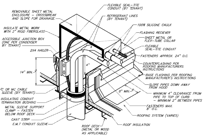
9 CONDENSER REFRIGERANT LINE PIPING AND POWER THROUGH ROOF DECK SCALE: NONE
