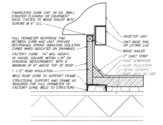
4 ROOF CURB DETAIL SCALE: NONE
