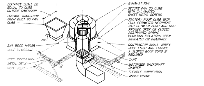
5 ROOF EXHAUST FAN DETAIL SCALE: NONE
