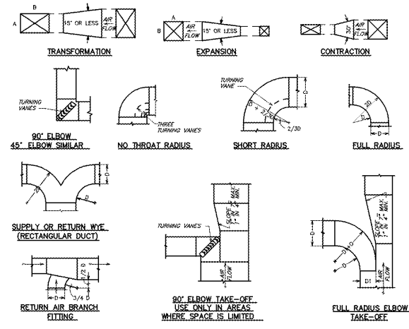
10 DUCTWORK DETAILS SCALE: NONE
