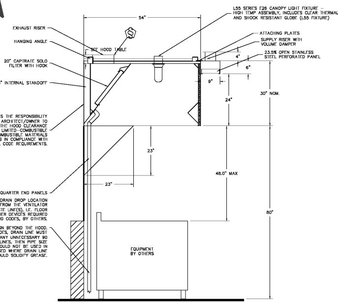
SECTION VIEW - MODEL 5430ND-2-PSP-FSS HOOD - #3 (GRILL)
