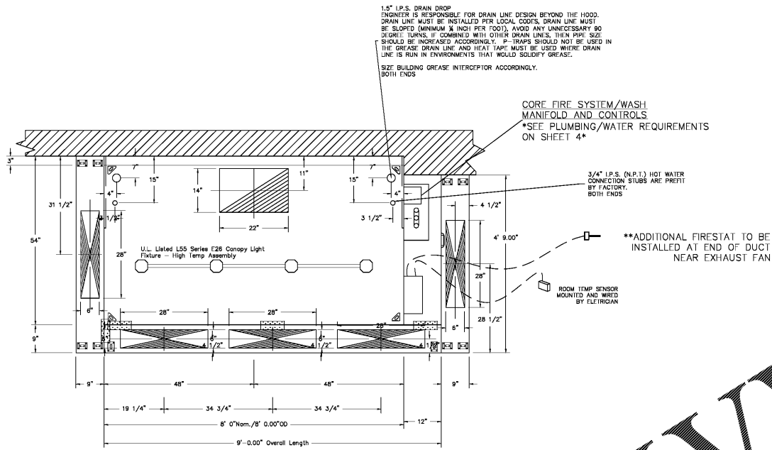
PLAN VIEW - Hood #3 (GRILL) 8' 0.00" LONG 5430ND-2-PSP-FSS
