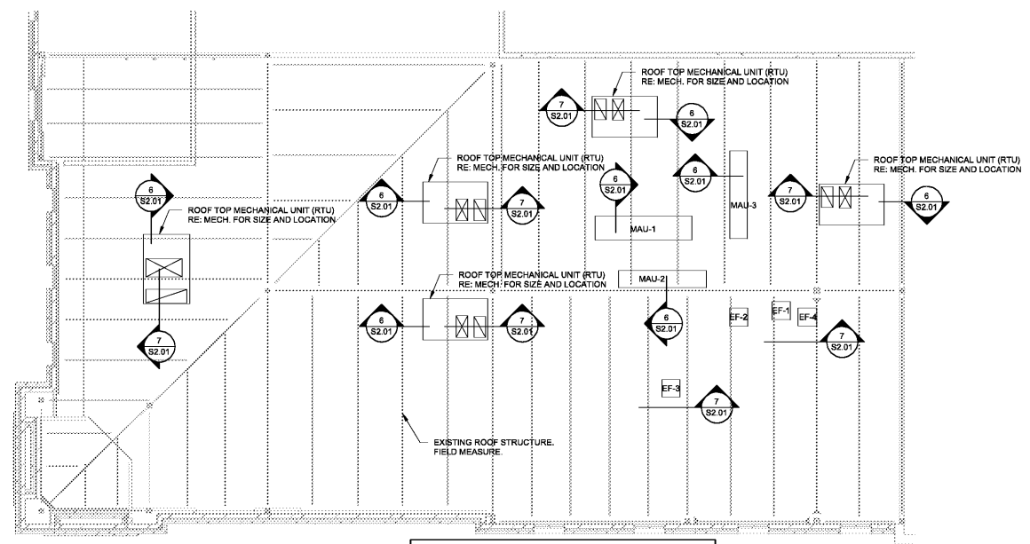
5 EXISTING ROOF FRAMING PLAN 1/8" = 1'-0"
