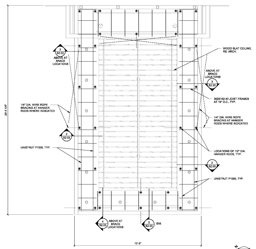
1 BAR SOFFIT PLAN 1/2" = 1'-0"
