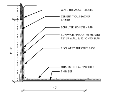
11 TYP. QUARRY TILE BASE DETAIL AT TILE WALL IN KITCHEN 7-1/2"
