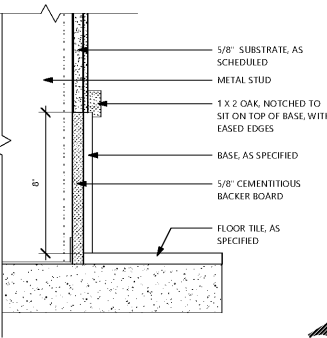
10 TYPICAL WAINSCOT BASE DETAIL 7-1/2"
