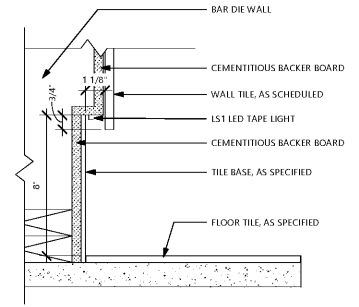
17 BASE DETAIL AT BAR FRONT 7-1/2"
