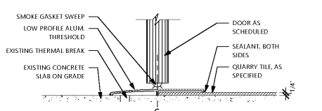
3 THRESHOLD AT REAR KITCHEN DOOR 7-1/2"
