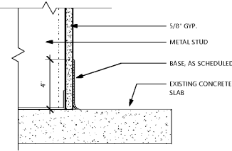
15 RUBBER BASE DETAIL IN MECH. CLOSET 7-1/2"
