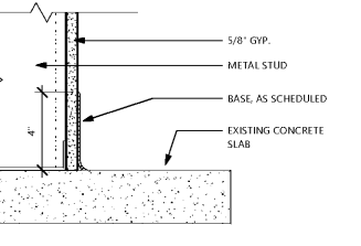
15 RUBBER BASE DETAIL IN MECH. CLOSET 7-1/2"
