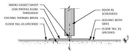
6 THRESHOLD AT COOLER & REAR KITCHEN DOOR 7-1/2"
