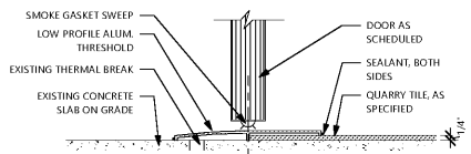
3 THRESHOLD AT REAR KITCHEN DOOR 7-1/2"
