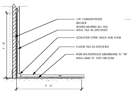
16 TILE WALL AND TILE FLOOR TRANSITION IN RESTROOM 7-1/2"
