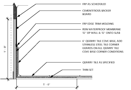
12 TYP. QUARRY TILE BASE DETAIL AT KITCHEN 7-1/2"
