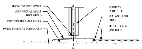
7 THRESHOLD AT PATIO DOOR 7-1/2"
