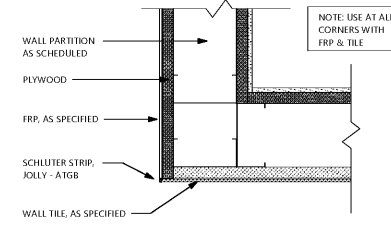
14 ENLARGED FRP TO TILE VERTICAL TRANSITION 7-1/2"
