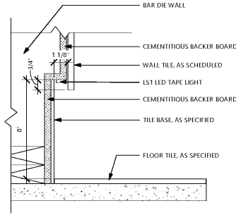
17 BASE DETAIL AT BAR FRONT 7-1/2"
