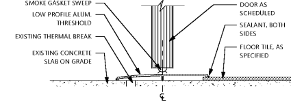
1 THRESHOLD AT STOREFRONT DOOR 7-1/2"
