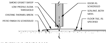
7 THRESHOLD AT PATIO DOOR 7-1/2"
