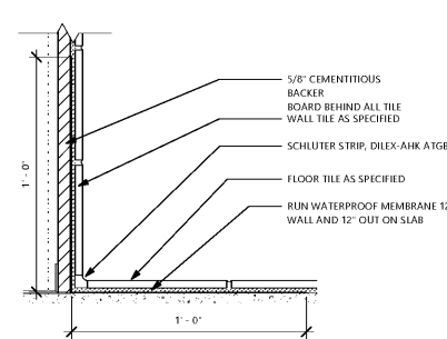
16 TILE WALL AND TILE FLOOR TRANSITION IN RESTROOM 7-1/2"
