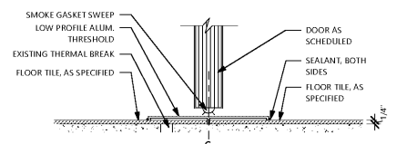
6 THRESHOLD AT COOLER & REAR KITCHEN DOOR 7-1/2"
