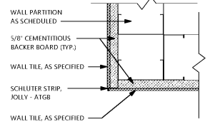
18 ENLARGED TILE TO TILE CORNER DETAIL 7-1/2"
