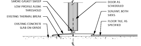
2 THRESHOLD AT STOREFRONT DOOR 7-1/2"
