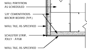
18 ENLARGED TILE TO TILE CORNER DETAIL 7-1/2"
