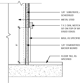
10 TYPICAL WAINGSCOT BASE DETAIL 7-1/2"
