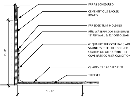
12 TYP. QUARRY TILE BASE DETAIL AT KITCHEN 7-1/2"
