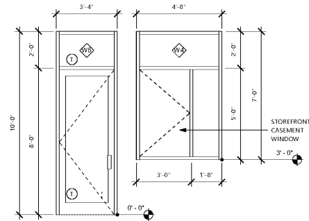
2 STOREFRONT ELEVATION 2 36'-1-0"
