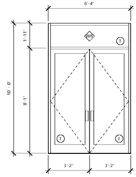
4 INTERIOR VESTIBULE STOREFRONT 36'-1-0"
