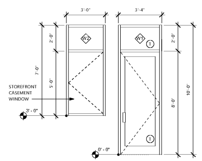
1 STOREFRONT ELEVATION 1 36'-1-0"
