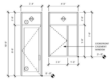
2 STOREFRONT ELEVATION 2 36'-1-0"
