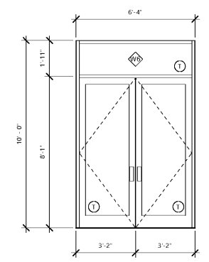
4 INTERIOR VESTIBULE STOREFRONT 36'-1-0"
