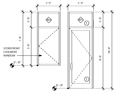
1 STOREFRONT ELEVATION 1 36'-1-0"
