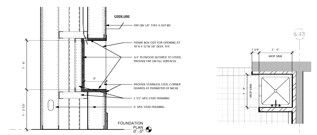
2 COOKLINE NICHE 2 11/16"
