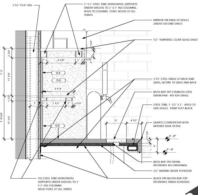
4 BACK BAR SECTION AT TAPS 1:6
