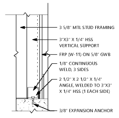
8 BASE DETAIL 1:2" = 1'-0"
