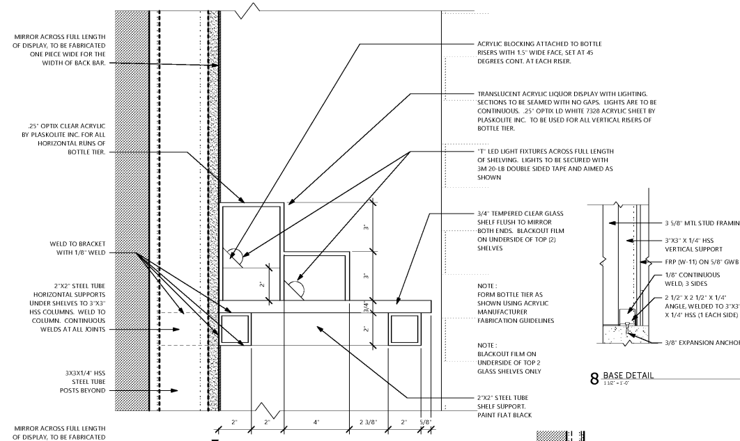
7 BACK BAR LIQUOR DISPLAY DETAIL 1:5
