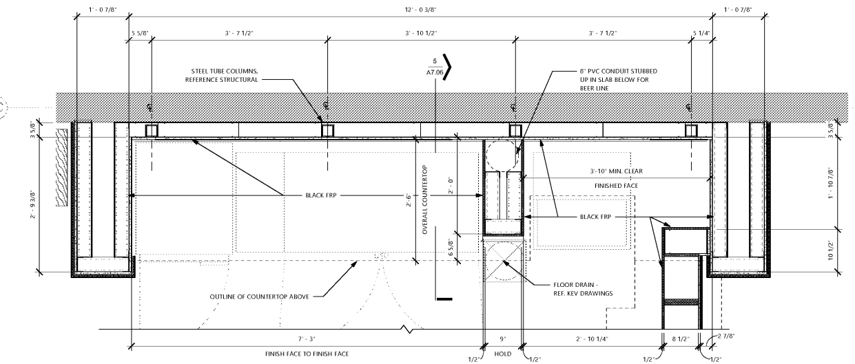
1 ENLARGED PLAN - BACK BAR 1:3.6
