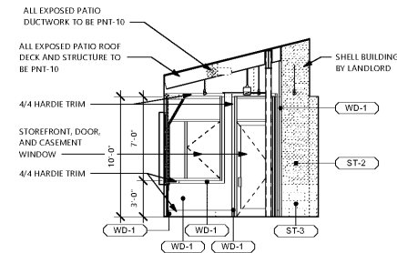
21 PATIO INTERIOR ELEVATION 3
