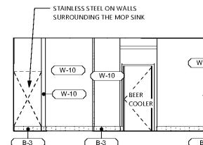
11 KITCHEN ELEVATION 7
