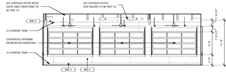
22 PATIO INTERIOR ELEVATION 4
