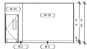
18 KITCHEN ELEVATION 14
