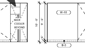
15 KITCHEN ELEVATION 11
