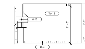
6 KITCHEN ELEVATION 2
