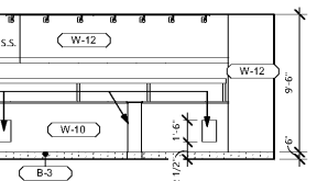
4 BEVERAGE RM ELEVATION 4
