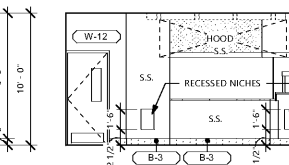
5 KITCHEN ELEVATION 1
