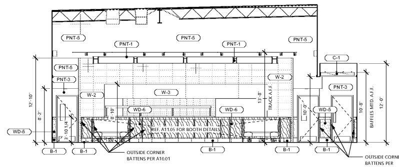
2 MAIN DINING ELEVATION 2 3/8" = 1'-0"
