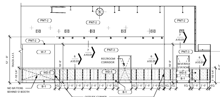
1 MAIN DINING ELEVATION 1 3/8" = 1'-0"
