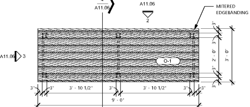
1 ENLARGED PLAN - COMMUNITY TABLE 1/8" = 1'-0"
