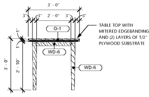
4 COMMUNITY TABLE SECTION 1/8" = 1'-0"
