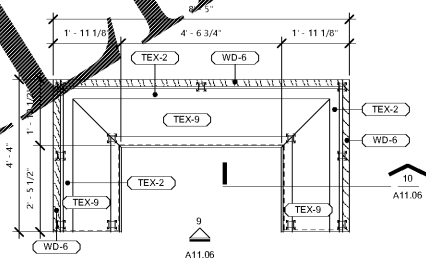
8 ENLARGED PLAN - U BOOTH 1/8" = 1'-0"
