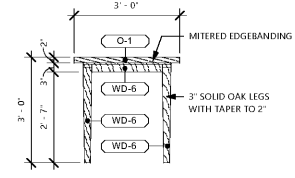
3 COMMUNITY TABLE SIDE ELEVATION 1/8" = 1'-0"
