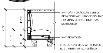
7 CIRCLE BOOTH SECTION 1/8" = 1'-0"
