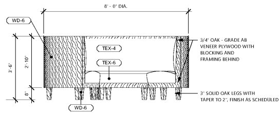
6 CIRCLE BOOTH ELEVATION 1/8" = 1'-0"
