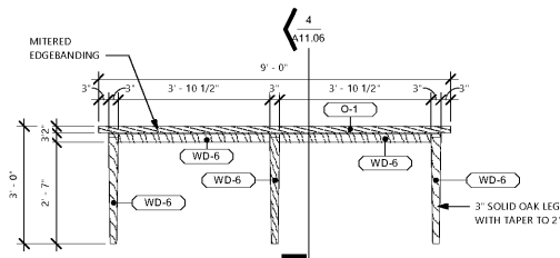
2 COMMUNITY TABLE FRONT ELEVATION 1/8" = 1'-0"
