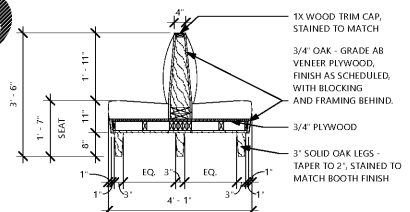
8 TYP. DOUBLE BOOTH SECTION 1 1/2" = 1'-0"
