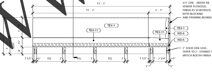
10 - BANQUETTE - FRONT ELEVATION 1/2" = 1'-0"
