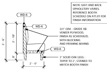
3 SINGLE BOOTH SIDE ELEVATION 1/2" = 1'-0"
