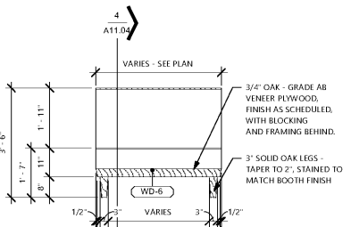
2 SINGLE BOOTH FRONT ELEVATION 1/2" = 1'-0"
