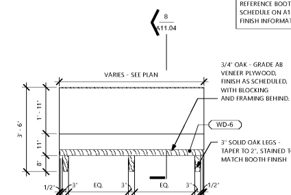
6 TYP. DOUBLE BOOTH ELEVATION A 1/2" = 1'-0"
