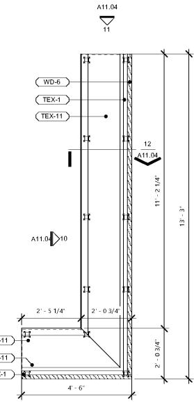
9 ENLARGED PLAN - TYP. L - BANQUETTE 1/2" = 1'-0"
