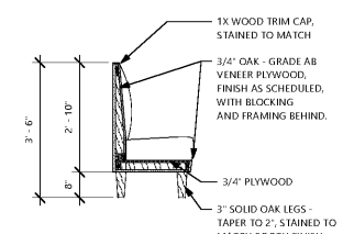
4 SINGLE BOOTH SECTION 1/2" = 1'-0"
