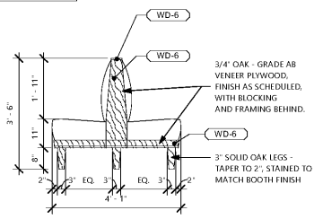
7 TYP. DOUBLE BOOTH ELEVATION B 1/2" = 1'-0"
