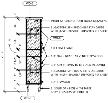
16 LIQUOR STORAGE SECTION 1/2" = 1'-0"
