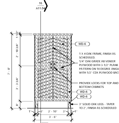
14 LIQUOR STORAGE FRONT ELEVATION 1/2" = 1'-0"
