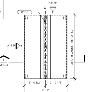
5 ENLARGED PLAN - TYP. DOUBLE BOOTH 1/2" = 1'-0"
