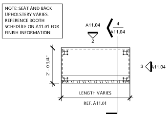
1 ENLARGED PLAN - TYP. SINGLE BOOTH 1/2" = 1'-0"
