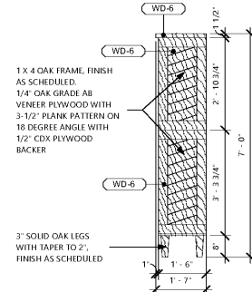
15 LIQUOR STORAGE SIDE ELEVATION 1/2" = 1'-0"
