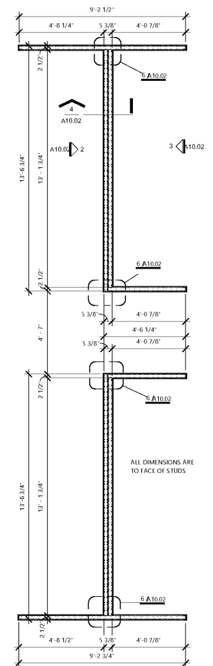
1 ENLARGED PLAN - BOOTH/DIVIDER WALL 3/2'-1/2"
