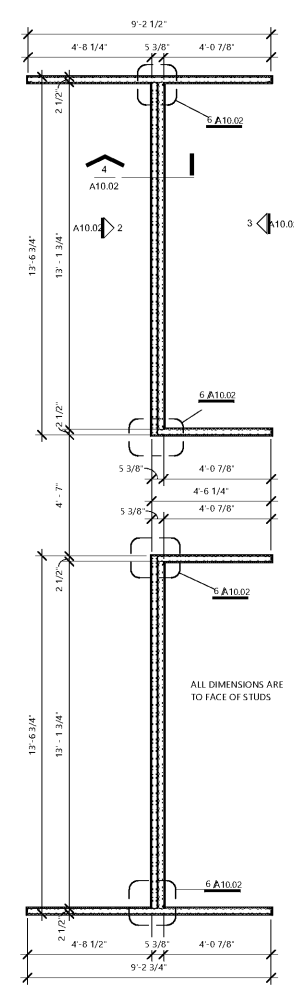
1 ENLARGED PLAN - BOOTH/DIVIDER WALL
