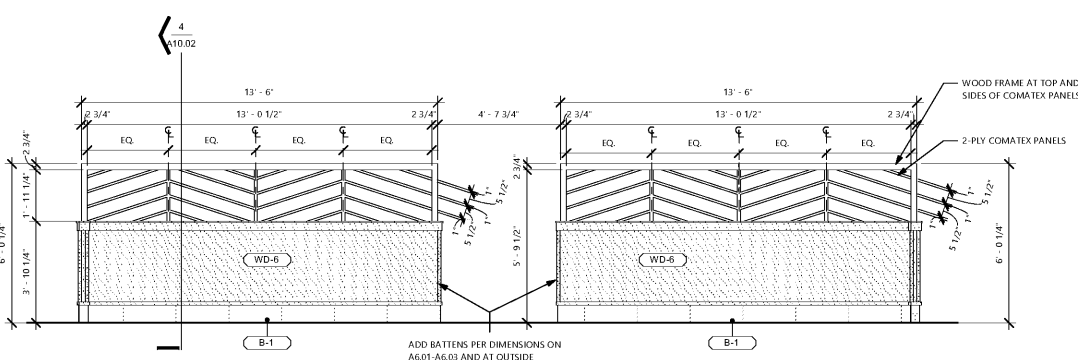
2 DIVIDER WALL ELEVATION - BANQUETTE SIDE
