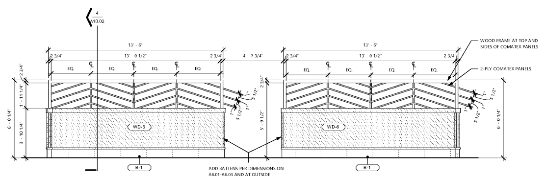
2 DIVIDER WALL ELEVATION - BANQUETTE SIDE 3/2'-1/2"
