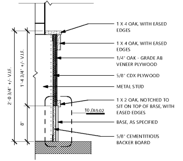
2 TYPICAL WAINSCOT SECTION - UNDER WINDOW 1/8\"/>
