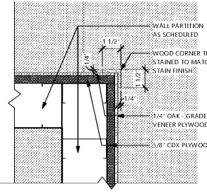
5 WAINSCOT CORNER DETAIL
