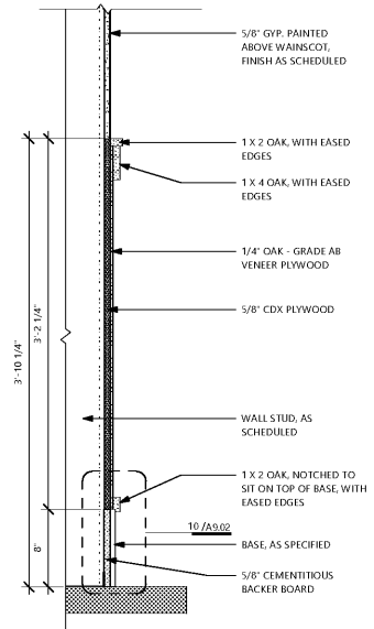
1 TYPICAL WAINSCOT SECTION 1/8\"/>
