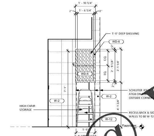
10 BUILT-IN SHELVING ELEVATION
