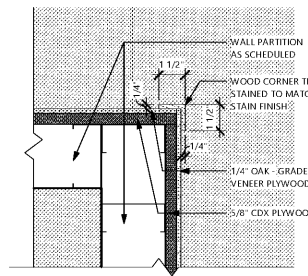
5 WAINSCOT CORNER DETAIL 1/8\"/>
