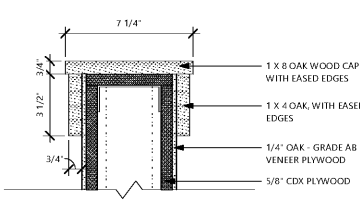
4 TYPICAL MILLWORK WALL - WOOD CAP 1/8\"/>
