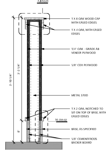
3 TYPICAL MILLWORK WALL
