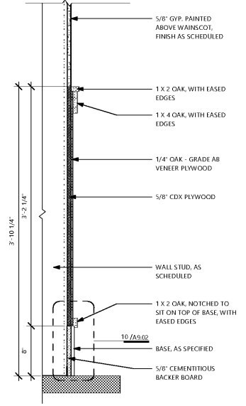
1 TYPICAL WAINSCOT SECTION
