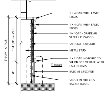
2 TYPICAL WAINSCOT SECTION - UNDER WINDOW
