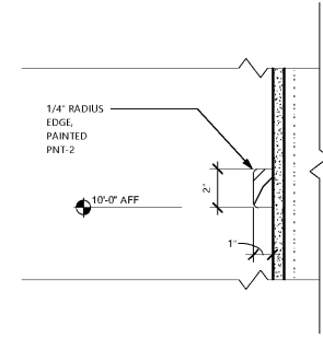
7 MATERIAL CHANGE TRIM DETAIL
