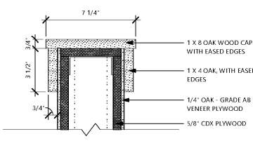
4 TYPICAL MILLWORK WALL - WOOD CAP
