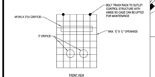
SECONDARY ORIFICE TRASH RACK NOT TO SCALE
