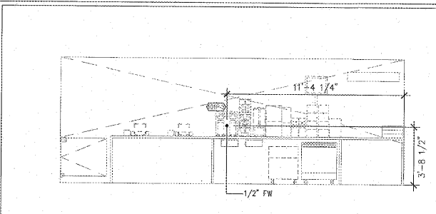
1 INTERIOR ELEVATION 4 AT DINING AREA
