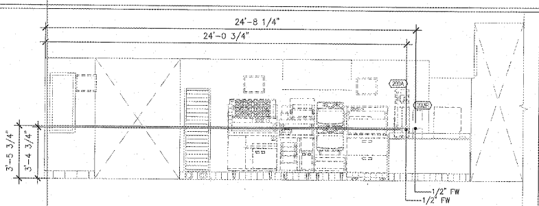
2 INTERIOR ELEVATION 6 AT KITCHEN AREA
