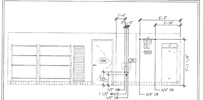
5 INTERIOR ELEVATION 10 AT PREP
