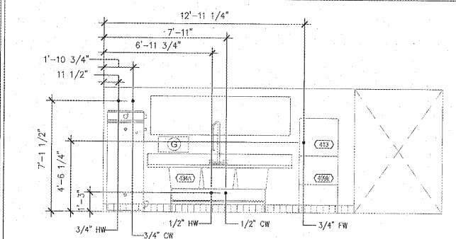
4 INTERIOR ELEVATION 9 AT DRIVE THRU
