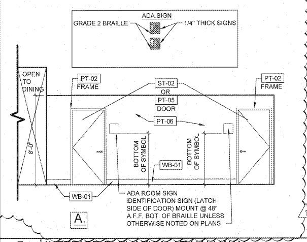
7 INTERIOR ELEVATION AT HALLWAY N.T.S. NOTE:
