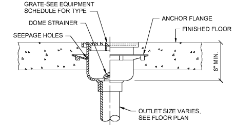
2 FLOOR SINK DETAIL P002 NOT TO SCALE
