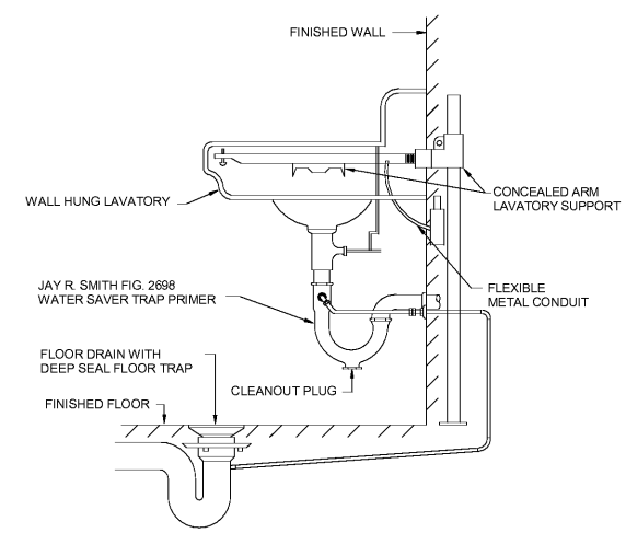
6 RESTROOM TRAP PRIMER DETAIL P002 NOT TO SCALE
