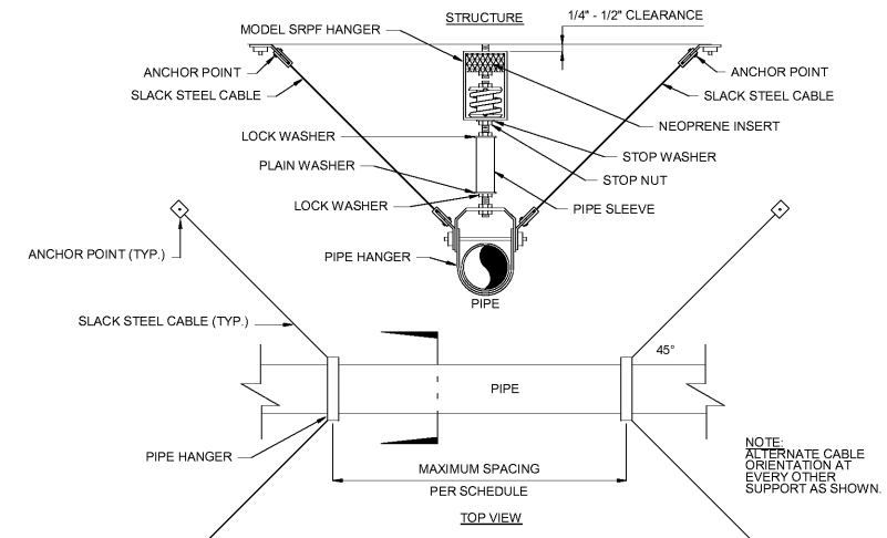
11 PIPE HANGER W/ SEISMIC RESTRAINTS P002 NOT TO SCALE
