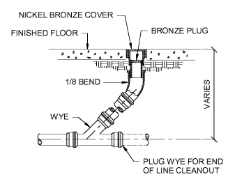
4 FLOOR CLEANOUT DETAIL P002 NOT TO SCALE
