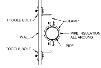
10 PIPE SUPPORT DETAILS P002 NOT TO SCALE
