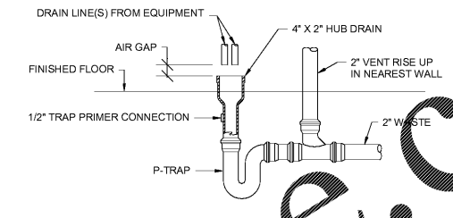
3 HUB DRAIN DETAIL P002 NOT TO SCALE
