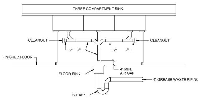
7 3 COMPARTMENT SINK DETAIL P002 NOT TO SCALE
