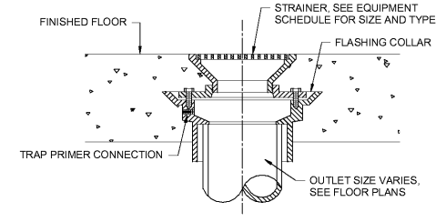
1 FLOOR DRAIN DETAIL P002 NOT TO SCALE
