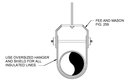
TYPE 2 TYPICAL FOR LINES NOT SUBJECT TO EXPANSION AND CONTRACTION.
