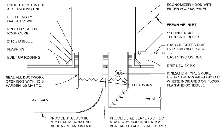
2 ROOFTOP UNIT WITH GAS HEAT NOT TO SCALE
