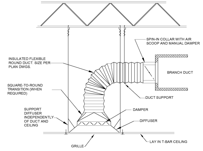
1 LAY-IN AIR DEVICE INSTALLATION DETAIL NOT TO SCALE
