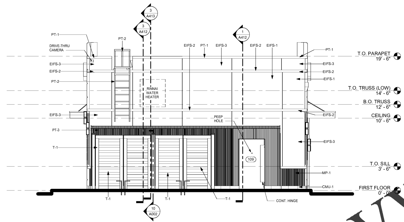
2 EXTERIOR ELEVATION - NORTH SCALE: 1/4" = 1'-0"
