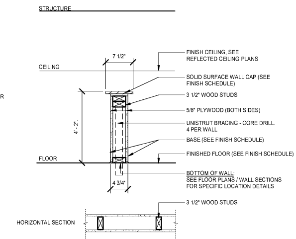
PARTITION TYPE 'W4'
