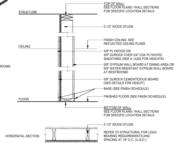
PARTITION TYPE 'W2'
