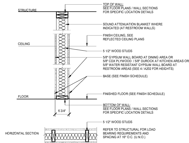
PARTITION TYPE 'W3'
