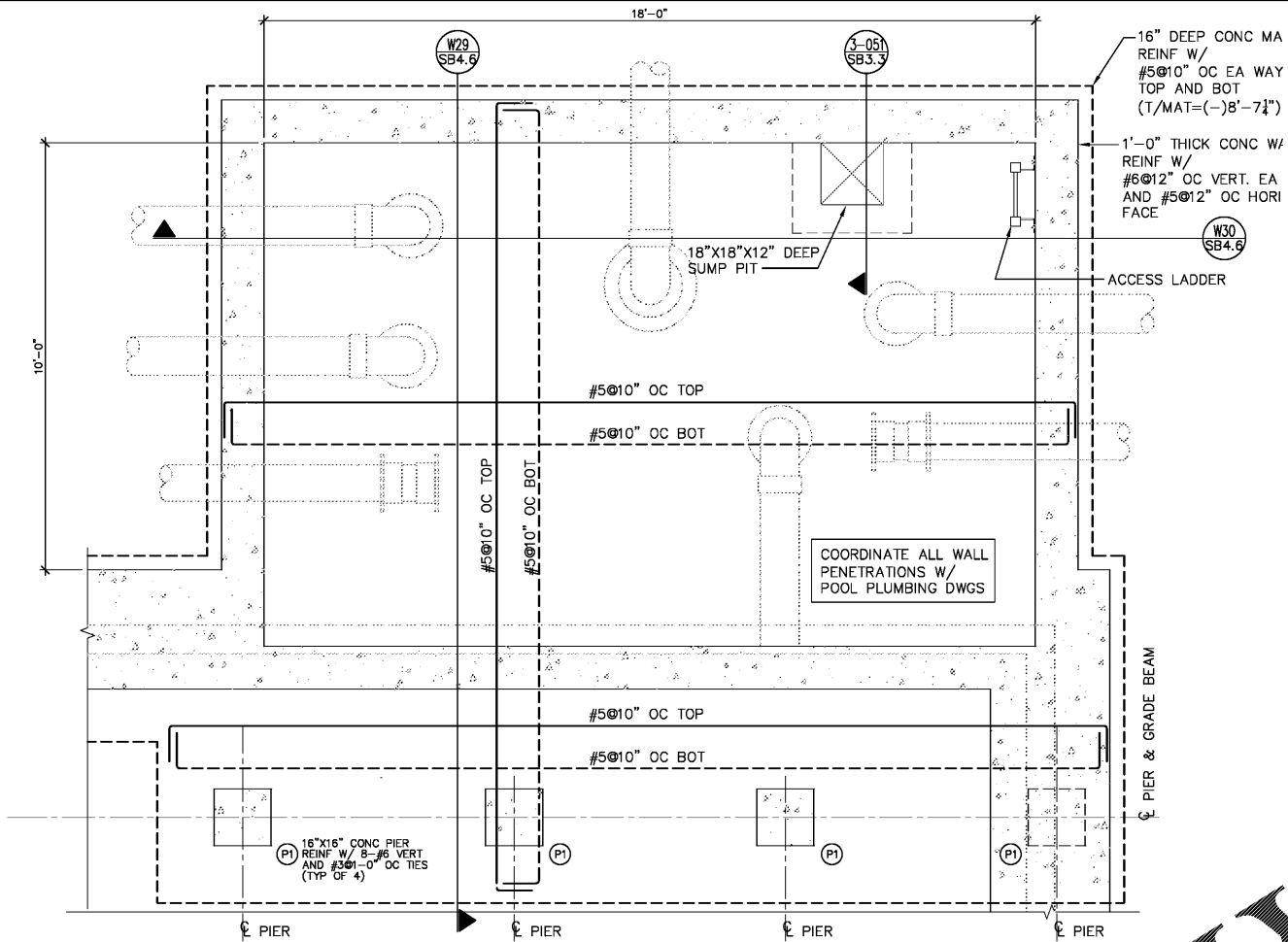
W28 LAZY RIVER POOL SURGE TANK - FOUNDATION PLAN SCALE: 1/2" = 1'-0"
