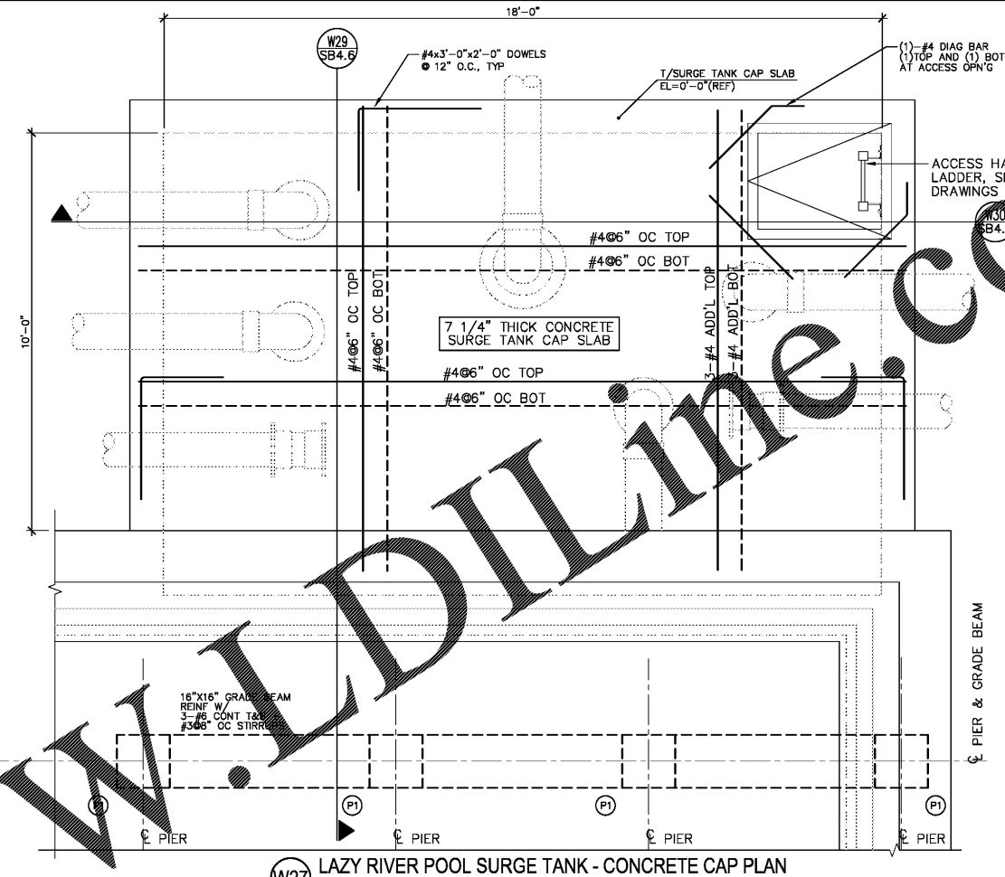
W27 LAZY RIVER POOL SURGE TANK - CONCRETE CAP PLAN SCALE: 1/2" = 1'-0"
