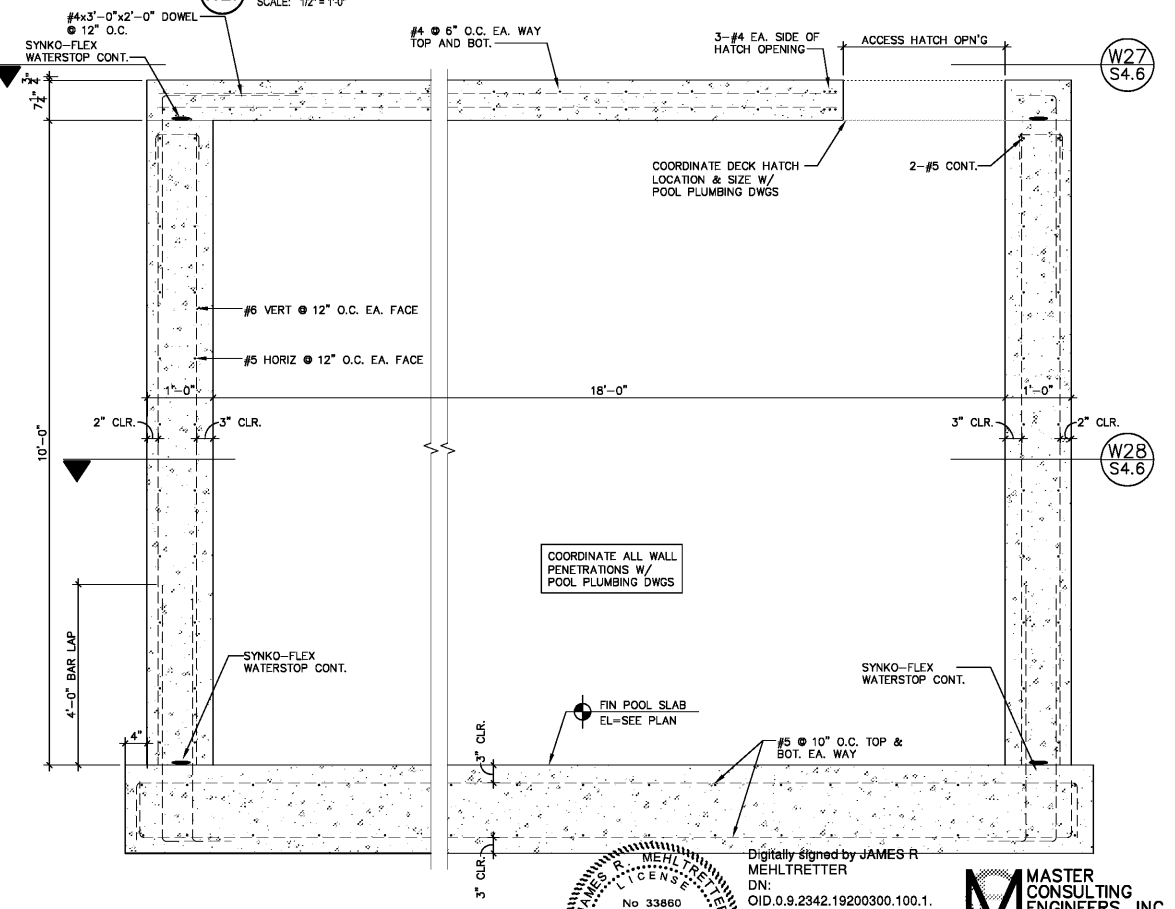
W30 LAZY RIVER POOL SURGE TANK - SECTION SCALE: 3/4" = 1'-0"
