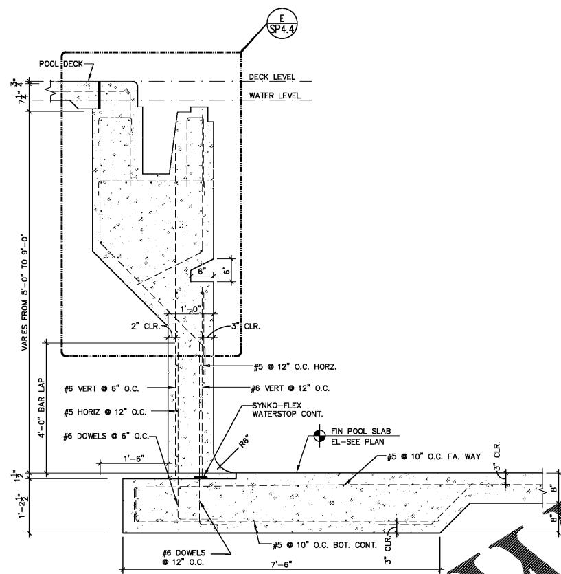
W16 COMPETITION POOL - WALL SECTION SCALE: 3/4" = 1'-0"
