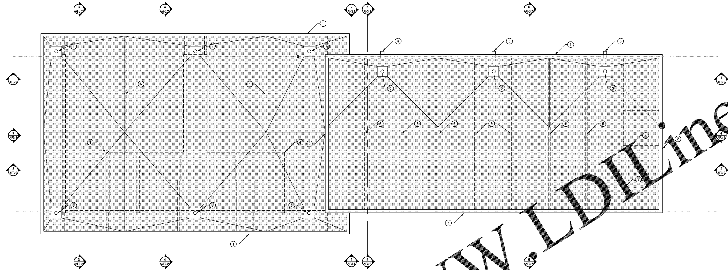
1 ROOF PLAN SCALE: 3/16" = 1'-0" 0 5 10 FEET
