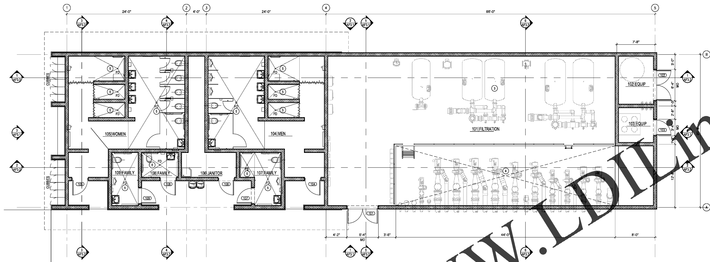
1 FLOOR PLAN SCALE: 3/16" = 1'-0" 0 5 10 FEET
