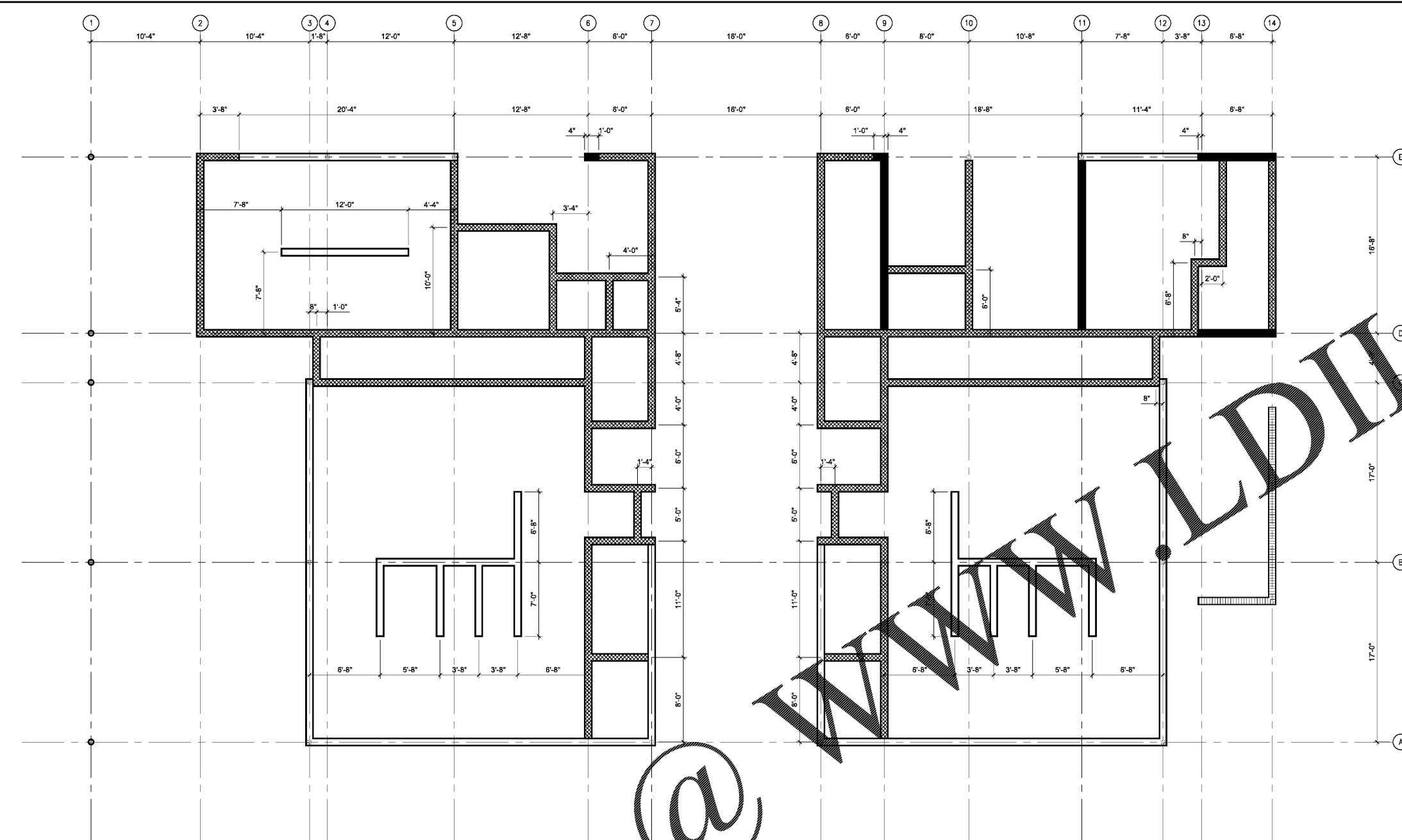
1 CMU WALL PLAN SCALE: 3/16" = 1'-0" 0 5 10 FEET
