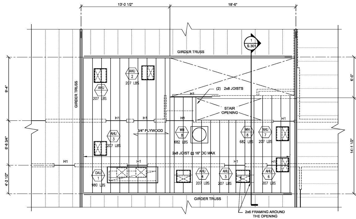
EQUIPMENT PLATFORM FRAMING PLAN S.102 1/4" = 1'-0"
