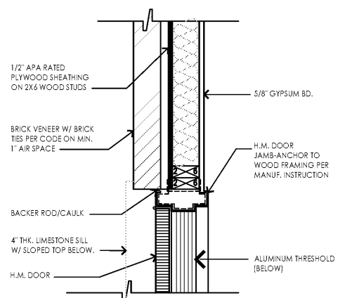
4 Section Thru H.M. Door Jamb Scale: 1-1/2" = 1'-0"
