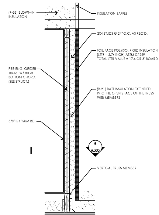
5 Typical Equipment Platform Wall Section Scale: 3/4" = 1'-0"
