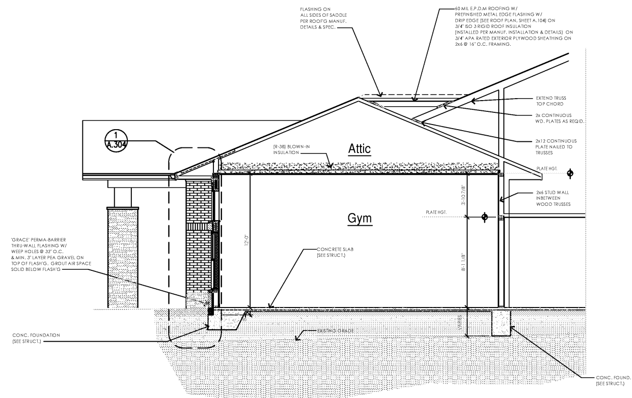
D A.301 Partial Building Section Scale: 1/4" = 1'-0"
