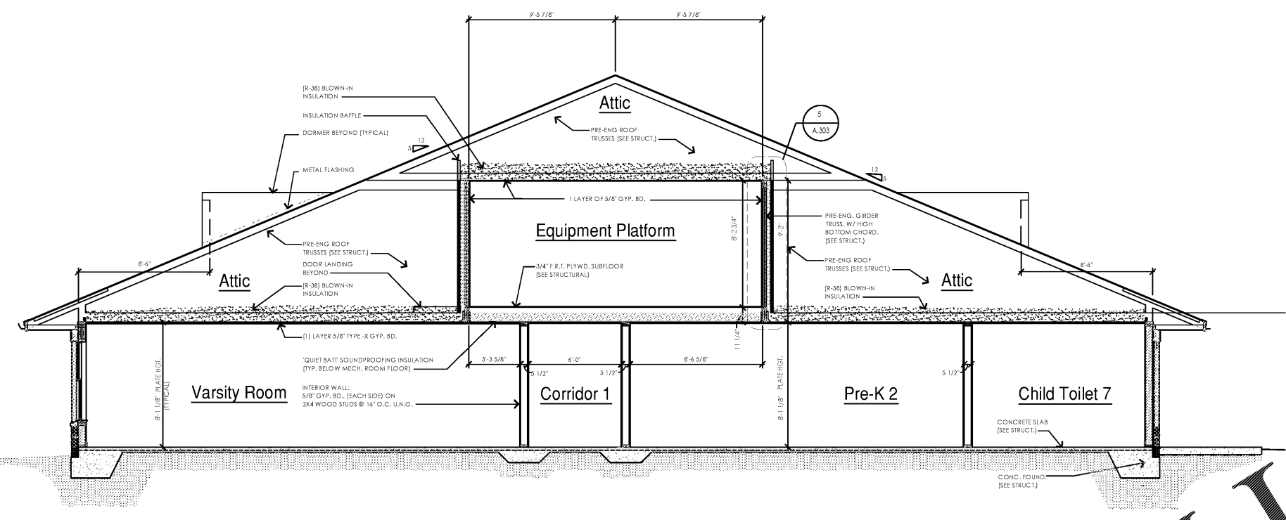
A A.300 Building Section Scale: 1/4" = 1'-0"
