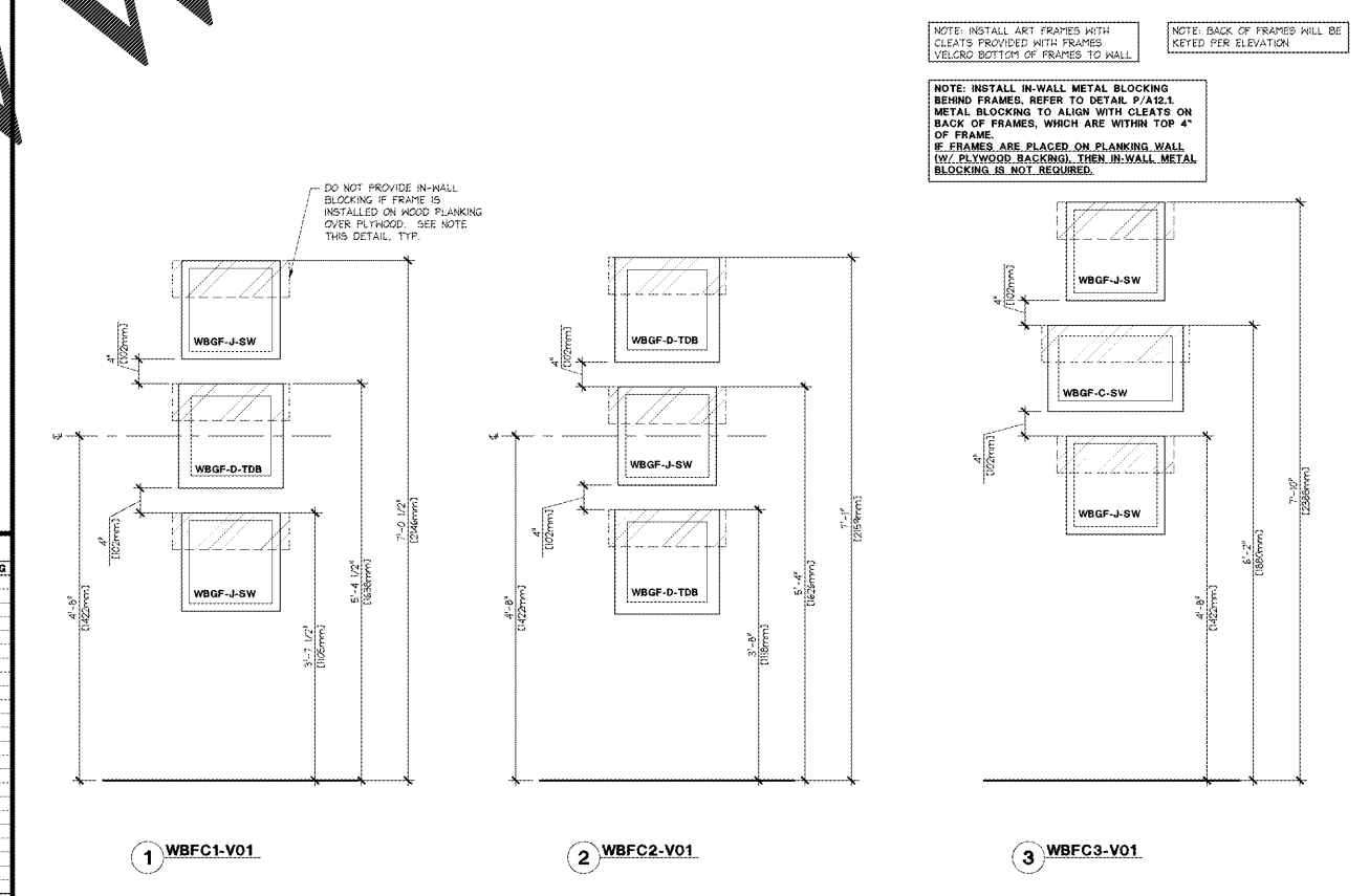
GRAPHIC FRAME LAYOUTS - SIS 1" = 1'-0" 42D-A118-A00-DET1 06.03.17
