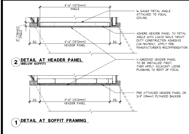
WIDE ANGLED DEMO SINK PLAN DETAIL AT PASS-THRU HEADER 3/4" x 1'-0" 42D-A113-001-DETL 10.06.17
