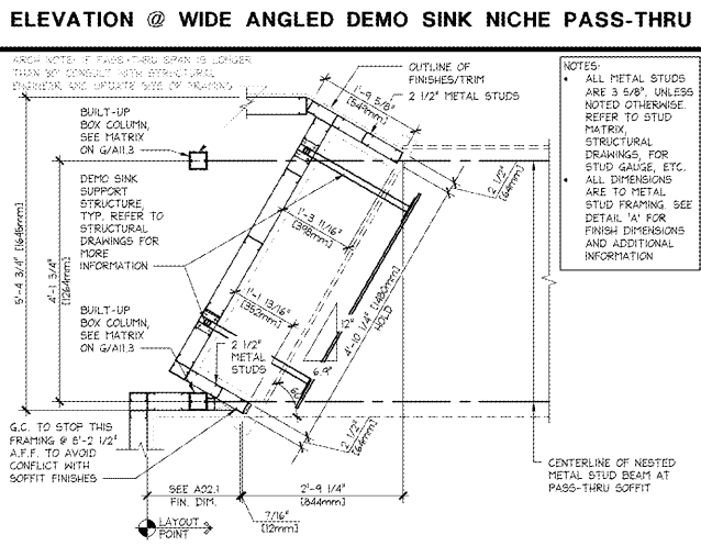
WIDE ANGLED DEMO SINK NICHE FRAMING PLAN - WITHOUT SHELVES 3/4" x 1'-0" 42D-A113-E03-DETL 10.23.17
