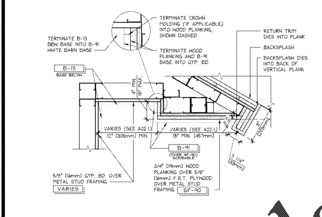
ELEVATION @ WIDE ANGLED DEMO SINK NICHE PASS-THRU - WITHOUT SHELVES 3/8" x 1'-0" 42E-A113-B05-ELEV 10.18.17
