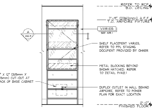
ELEVATION @ WHITE BARN ARMOIRE SMALL (WBARMS-V##-ST)
