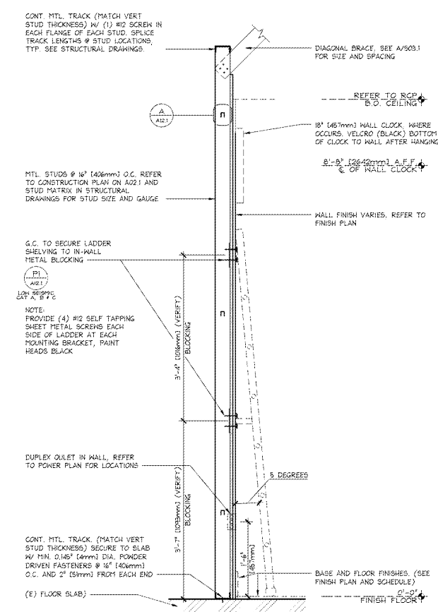
LADDER SHELVE SECTION
