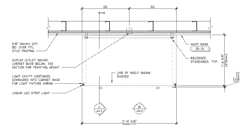
ENLARGED PLAN @ WHITE BARN ARMOIRE SMALL (WBARMS-V##-ST)
