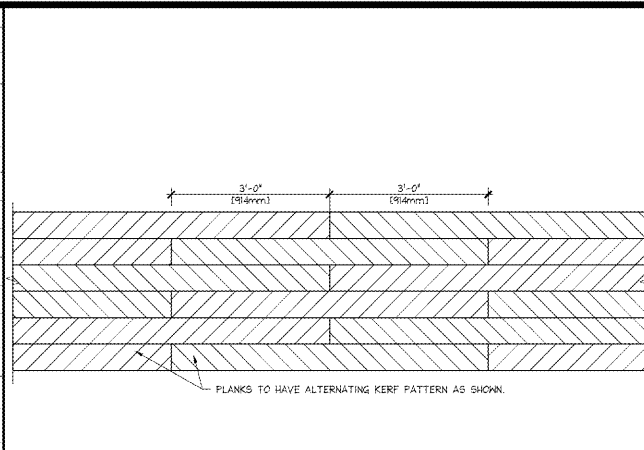
PATTERN OF PLANKING SF-90 @ CEILING
