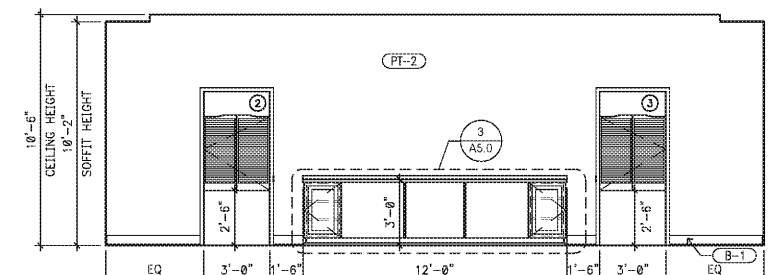
3 INTERIOR ELEVATION SCALE: 1/4" = 1'-0"
