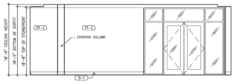
1 INTERIOR ELEVATION SCALE: 1/4" = 1'-0"
