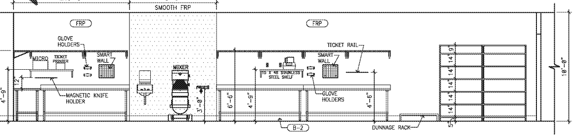
11 INTERIOR ELEVATION SCALE: 1/4" = 1'-0"
