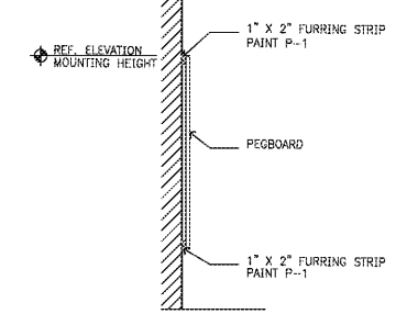
B PEGBOARD MOUNTING DETAIL SCALE: 1/2" = 1'-0"
