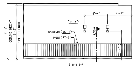
2 INTERIOR ELEVATION SCALE: 1/4" = 1'-0"
