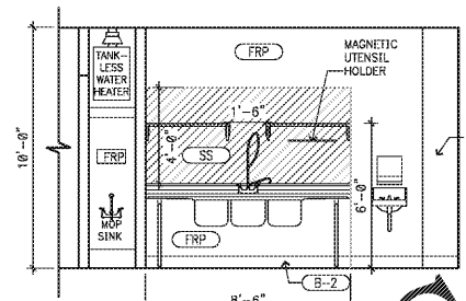
9 INTERIOR ELEVATION SCALE: 1/4" = 1'-0"
