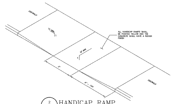
2 HANDICAP RAMP C112 NOTE: RAMP TO BE OUTLINED WITH 4" WHITE STRIPING.
