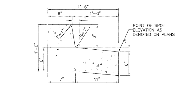
7 TYPICAL 18" REJECT CURB & GUTTER - SECTION C112
