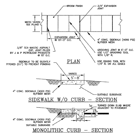
6 SIDEWALK - DETAIL C112 NOTE: CONTRACTOR TO VERIFY SUITABILITY AND COMPACTION OF NATIVE OR FILL SUBGRADE MATERIAL PRIOR TO INSTALLATION OF SIDEWALK.
