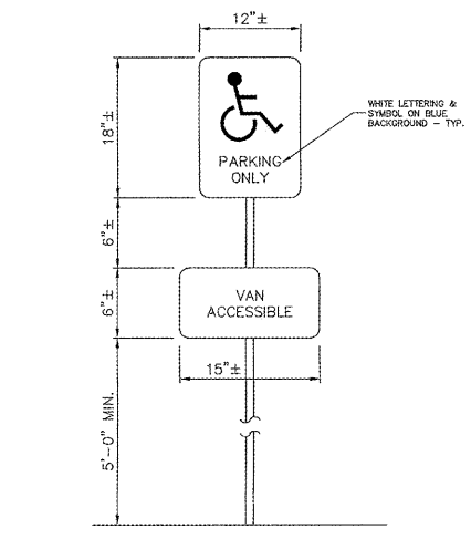
5 TYPICAL HANDICAPPED SIGN - ELEVATION C112
