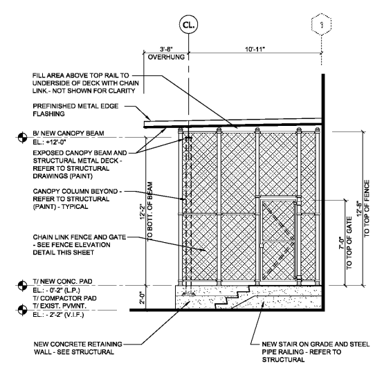
2 LOADING PLATFORM ELEVATION A4.3 SCALE: 1/4" = 1'-0"
