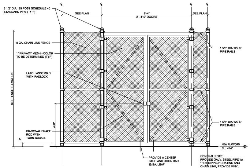
3 CHAIN LINK FENCE DETAIL AT GATE A4.3 SCALE: 1/2" = 1'-0"
