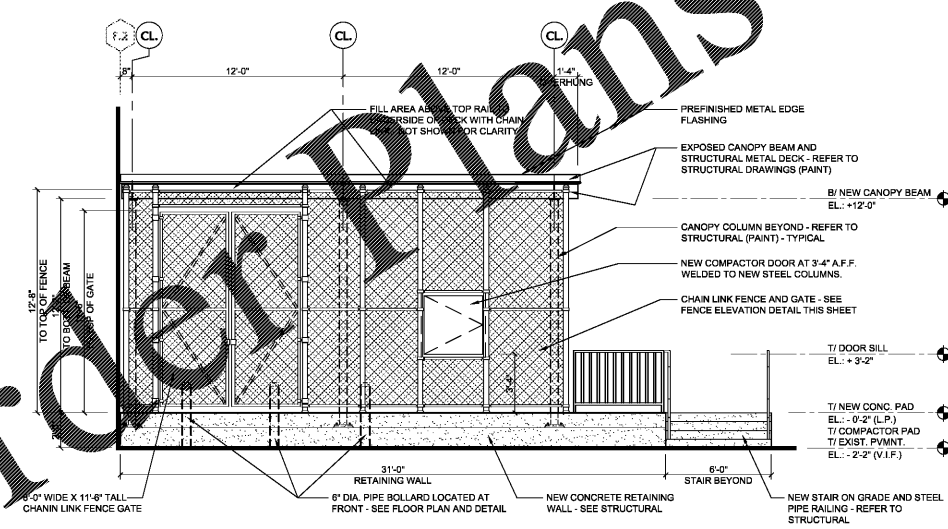
1 LOADING PLATFORM ELEVATION A4.3 SCALE: 1/4" = 1'-0"
