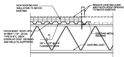
3 METAL DECK PATCH DETAIL A1.1a SCALE: NONE
