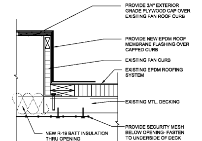
2 CURB PATCH DETAIL A1.1a SCALE: NONE
