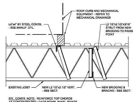
5 DETAIL AT R.T.U. SUPPORT A1.1a SCALE: NONE
