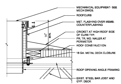
1 MECHANICAL CURB DETAIL A1.1a SCALE: NONE
