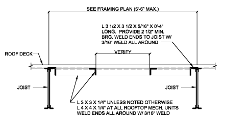
6 ROOF DECK OPENING DETAIL A1.1a SCALE: NONE
