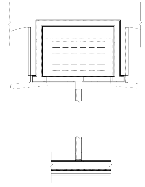
3 OPERABLE PARTITION DETAIL A4.14 3/4" x 1/0"
