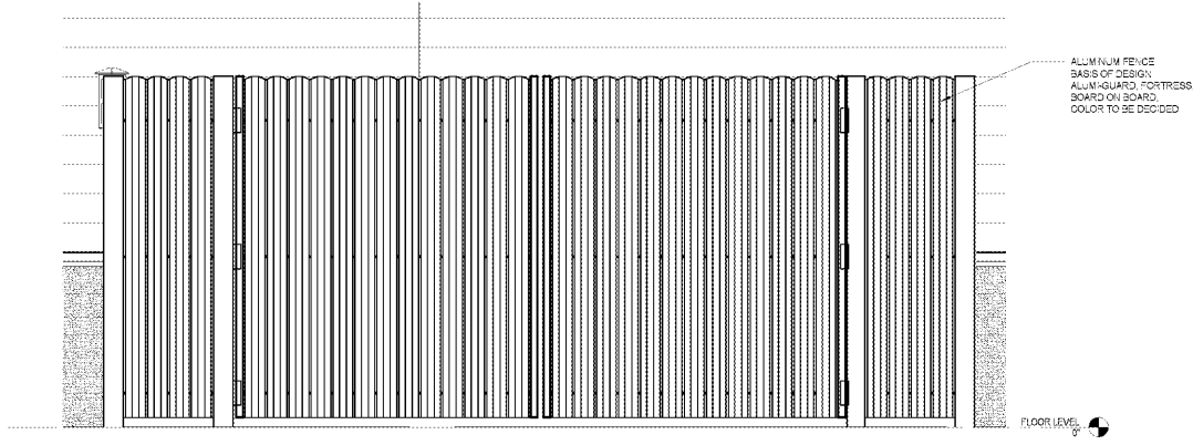
3 TYPICAL FENCE GATE ELEVATION A4.14 3/4" x 1/0"
