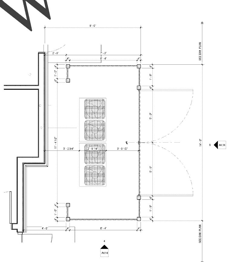
2 FENCE DETAIL - AREA 02 A4.14 1/2" x 1/0"
