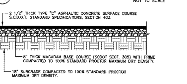
7B HEAVY DUTY ASPHALT NOT TO SCALE
