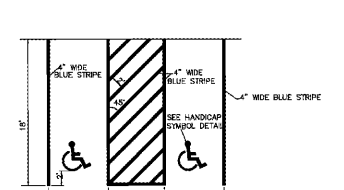
2 HANDICAP ACCESSIBLE PARKING STALLS NOT TO SCALE
