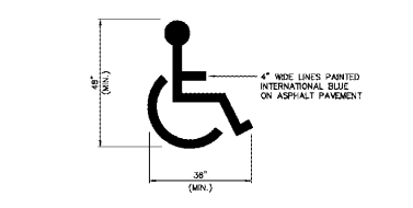
1 HANDICAP PARKING PAINTED SYMBOL NOT TO SCALE
