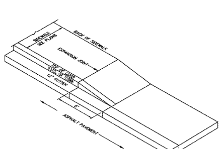
4 HANDICAP RAMP NOT TO SCALE
