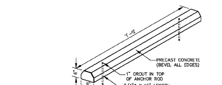
9 PRECAST CONCRETE WHEELSTOP NOT TO SCALE
