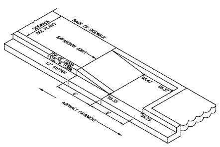
3 SIDEWALK ACCESS RAMP NOT TO SCALE
