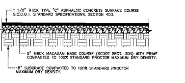
7A LIGHT DUTY ASPHALT NOT TO SCALE
