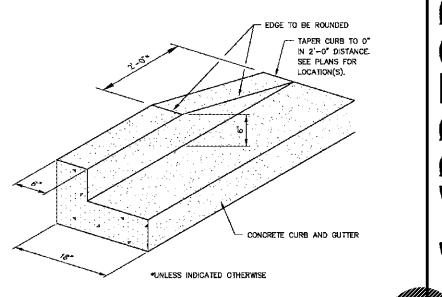
5 TAPERED CURB NOT TO SCALE
