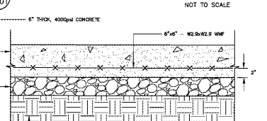
13 CONCRETE PAVEMENT EDGE NOT TO SCALE
