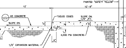
DUMPSTER PAD AND BOLLARDS SCALE: NOT TO SCALE
