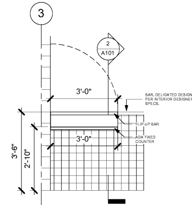
3 ADA BAR ELEVATION 1/2" = 1'-0"
