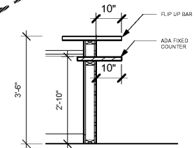
2 ADA BAR SECTION 1/2" = 1'-0"
