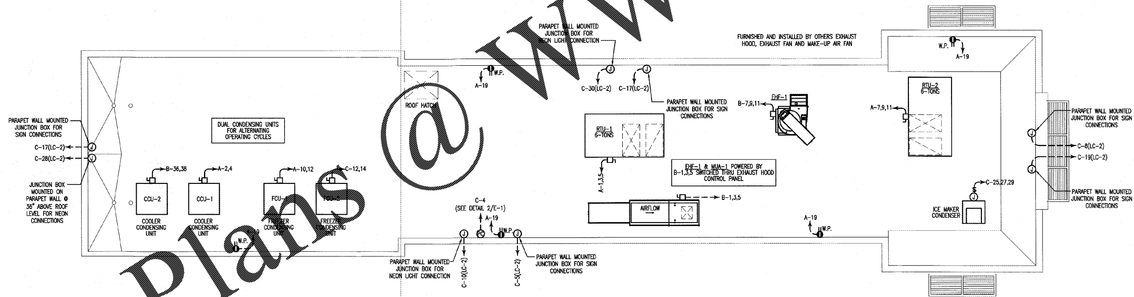
ROOF ELECTRICAL PLAN 1 E-3 SCALE: 1/4"=1'-0"
