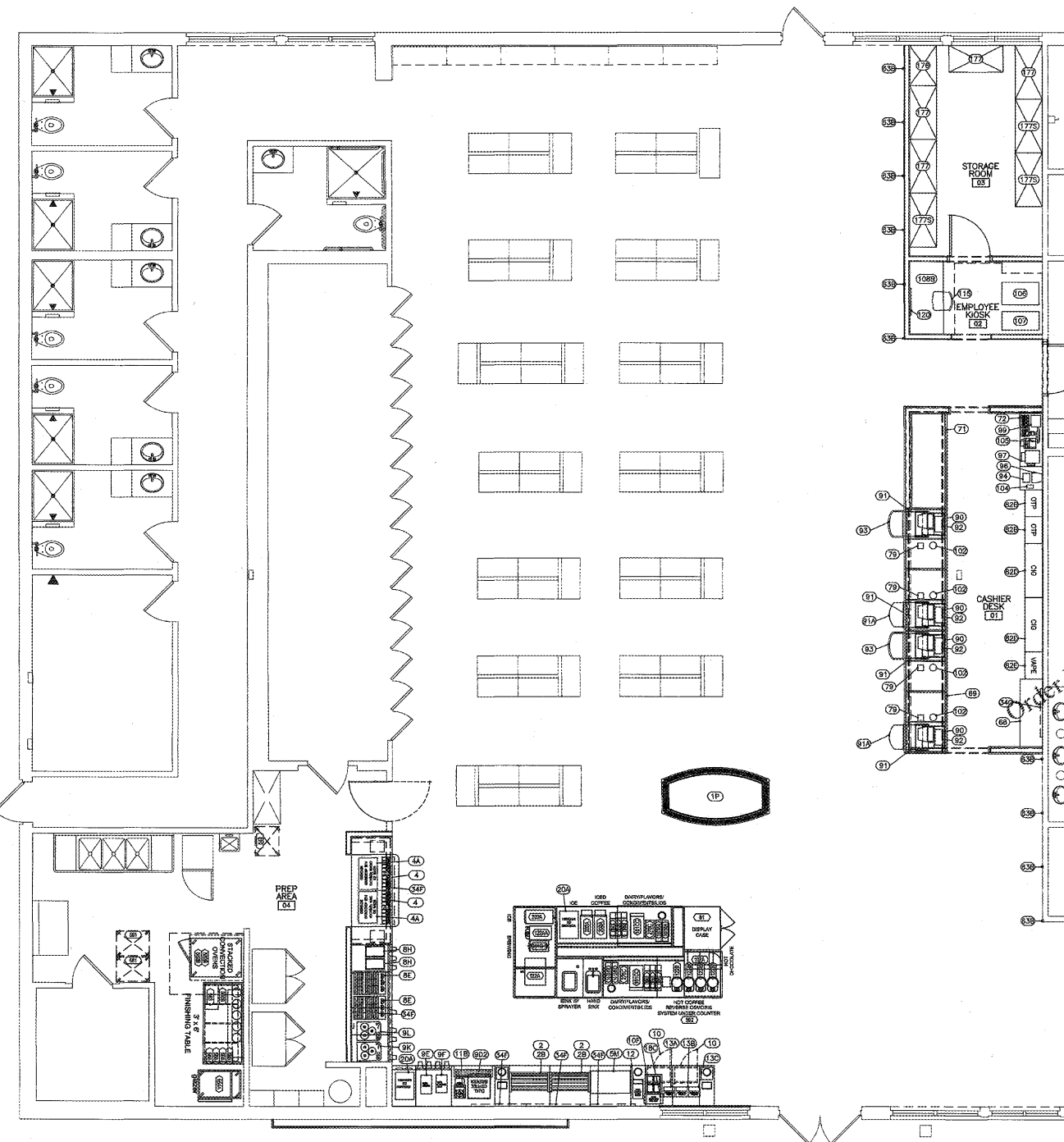
1 EQUIPMENT PLAN A5 3/16" = 1'-0"
