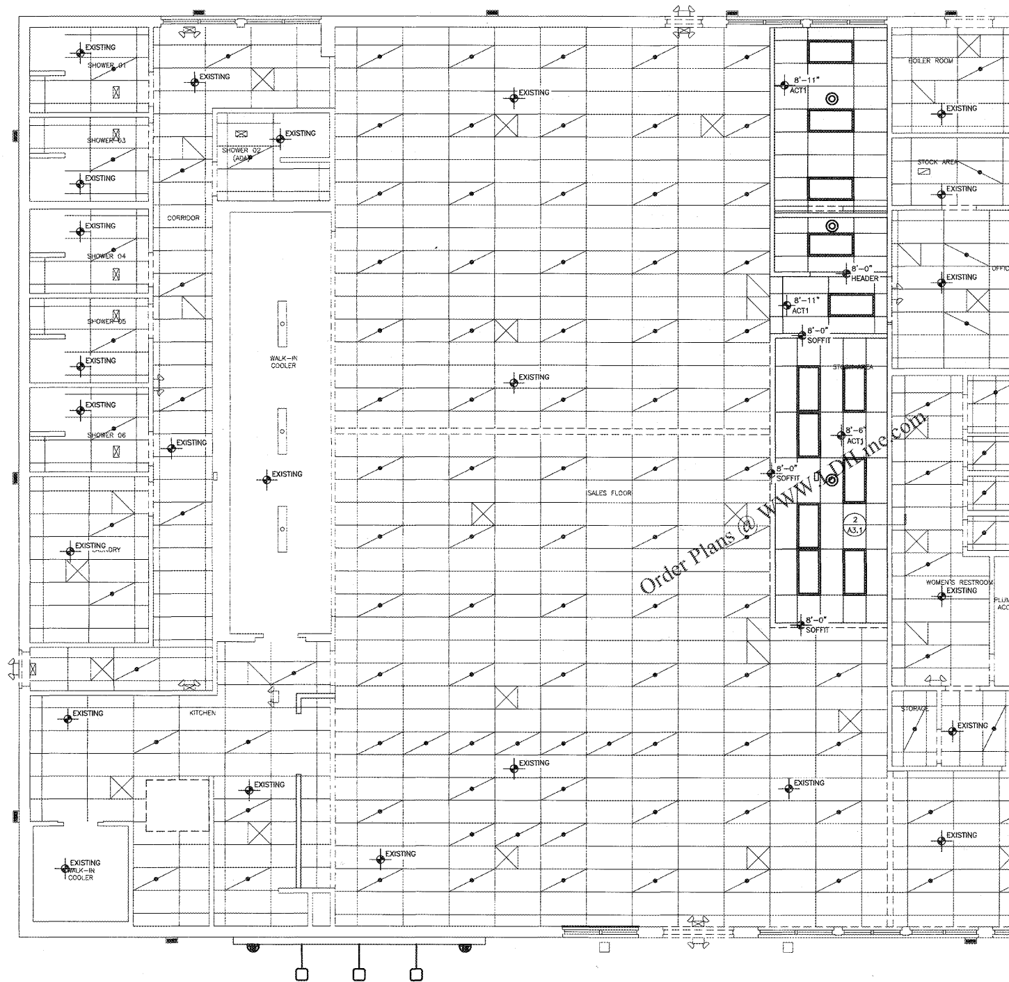
1 REFLECTED CEILING PLAN - RENOVATION A3.1 3/16" = 1'-0"
