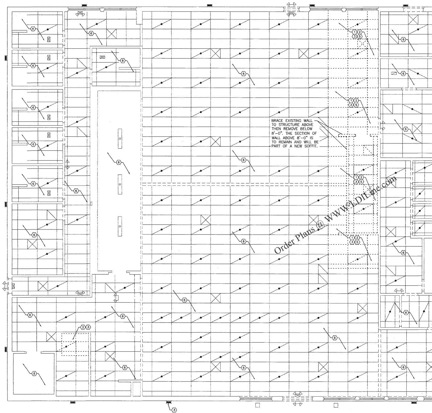
1 REFLECTED CEILING PLAN - DEMOLITION A3 3/16" = 1'-0"
